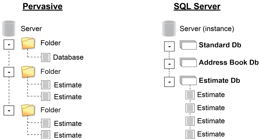
Figure 6: Comparison of Pervasive and SQL Server
